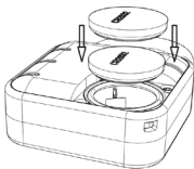
Anode face up and cathode face down
